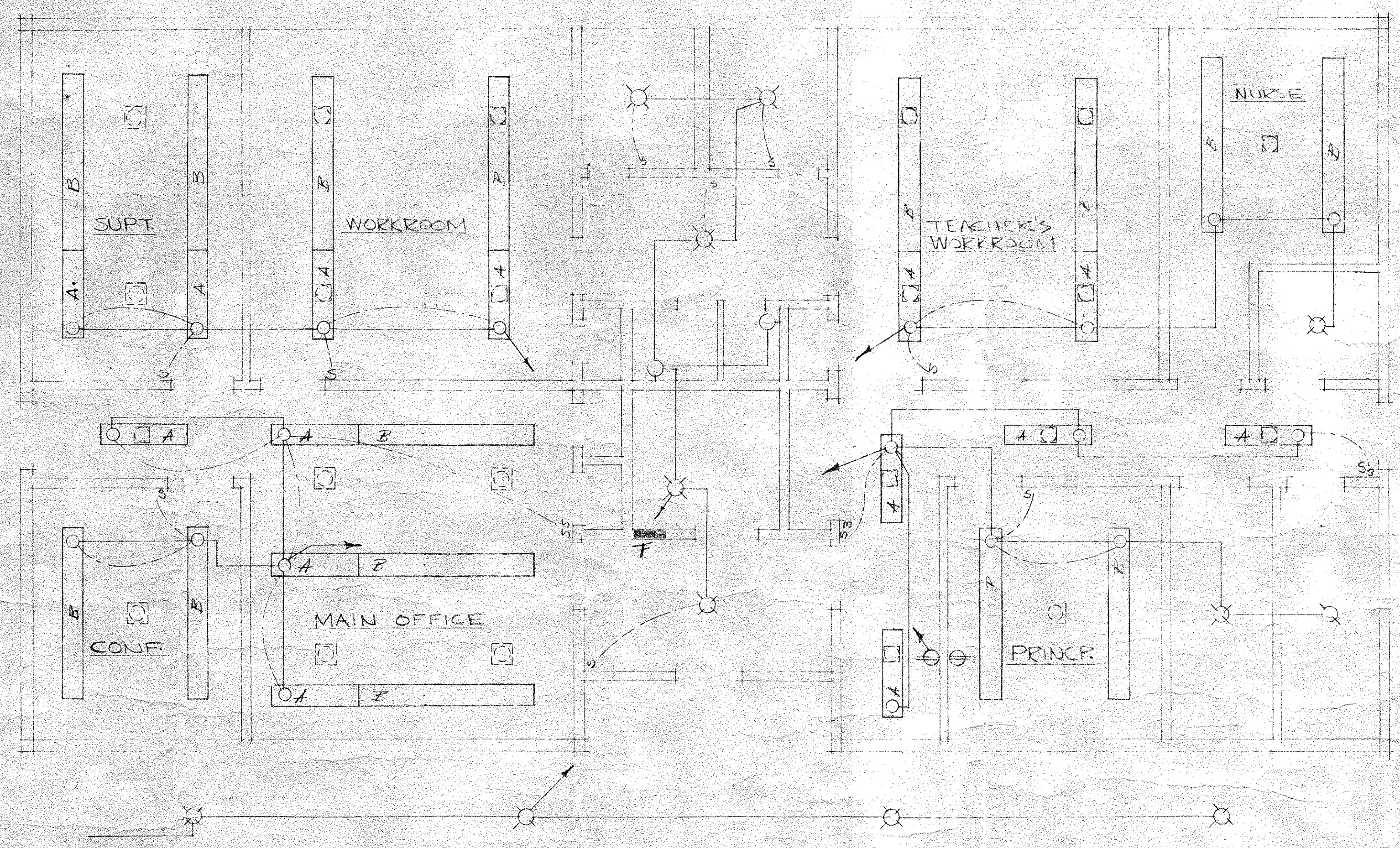
BLDG # 6 LIGHTING PLAN. SCALE 1/4" = 1'-0"
