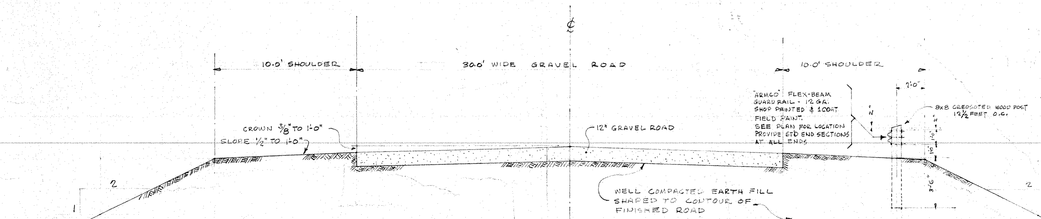
TYPICAL SECTION OF NEW ROAD SCALE \frac{1}{4} "=1'-0"
