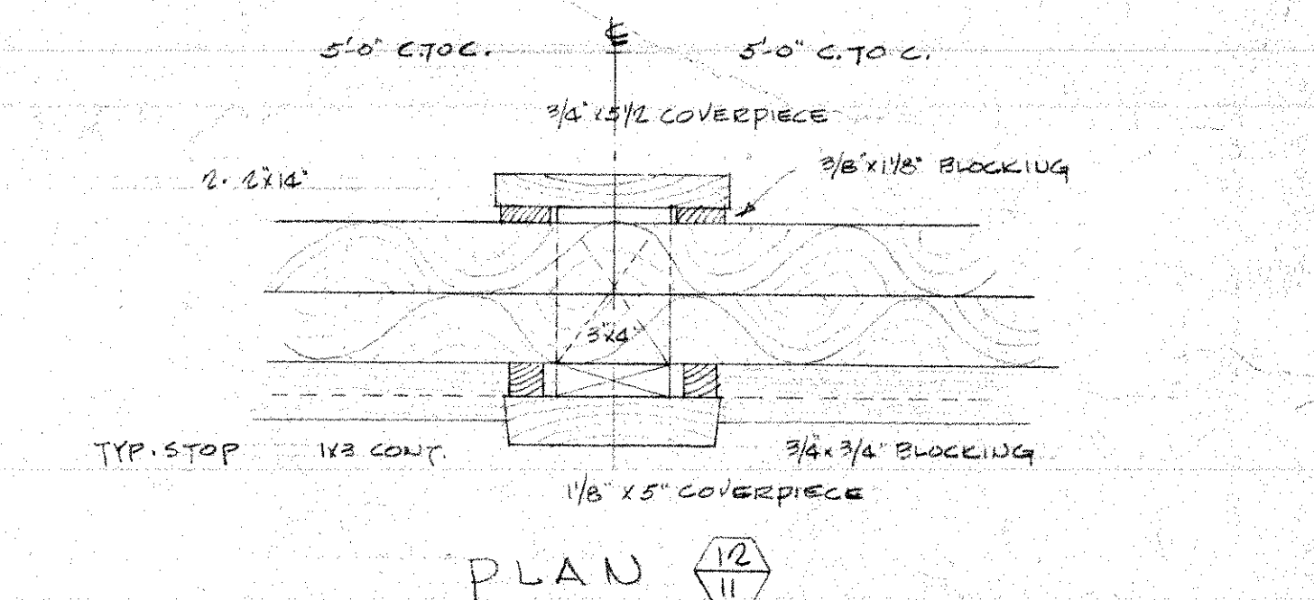
PLAN 12/11
