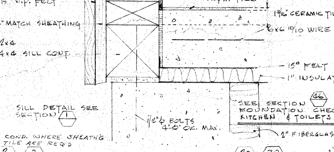
SECTION 18/8
