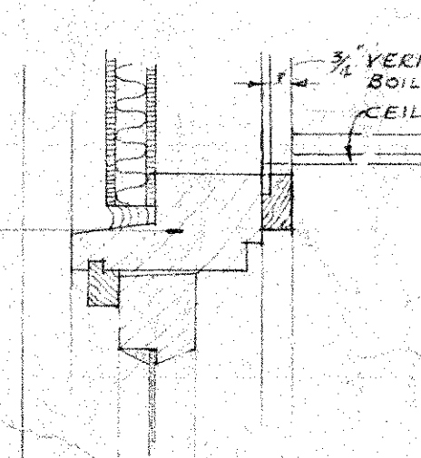
SECTION 23/8
