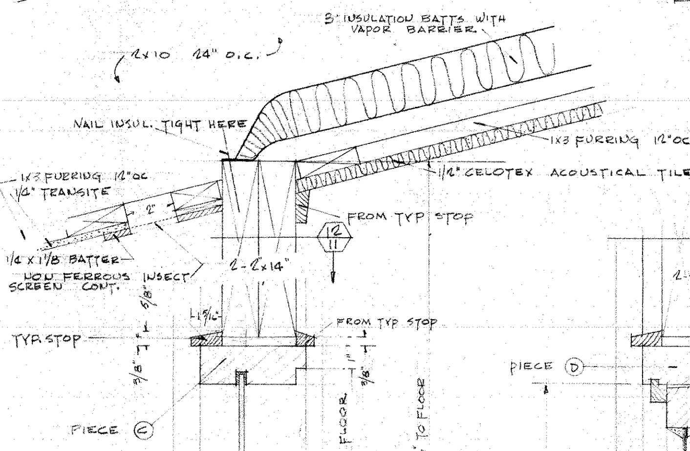
SECTION 9/8
