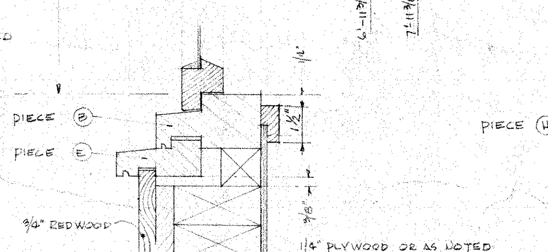
SECTION 16/8
