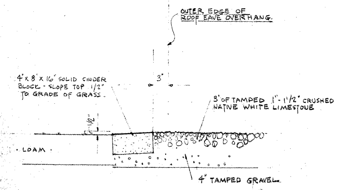
DETAIL OF CINDERBLOCK & LIMESTONE SURFACING UNDER ROOF OVERHANG SCALE: 1" = 1'-0"
